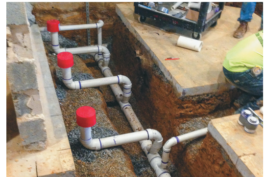
Underground piping.
